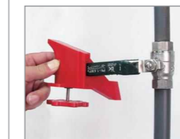
Step 1: Insert the ball valve handle
